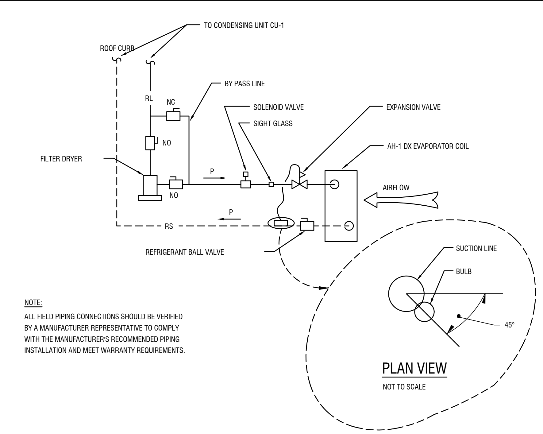
1 DX COOLING COIL PIPING DETAIL M8.2 SCALE: NTS
