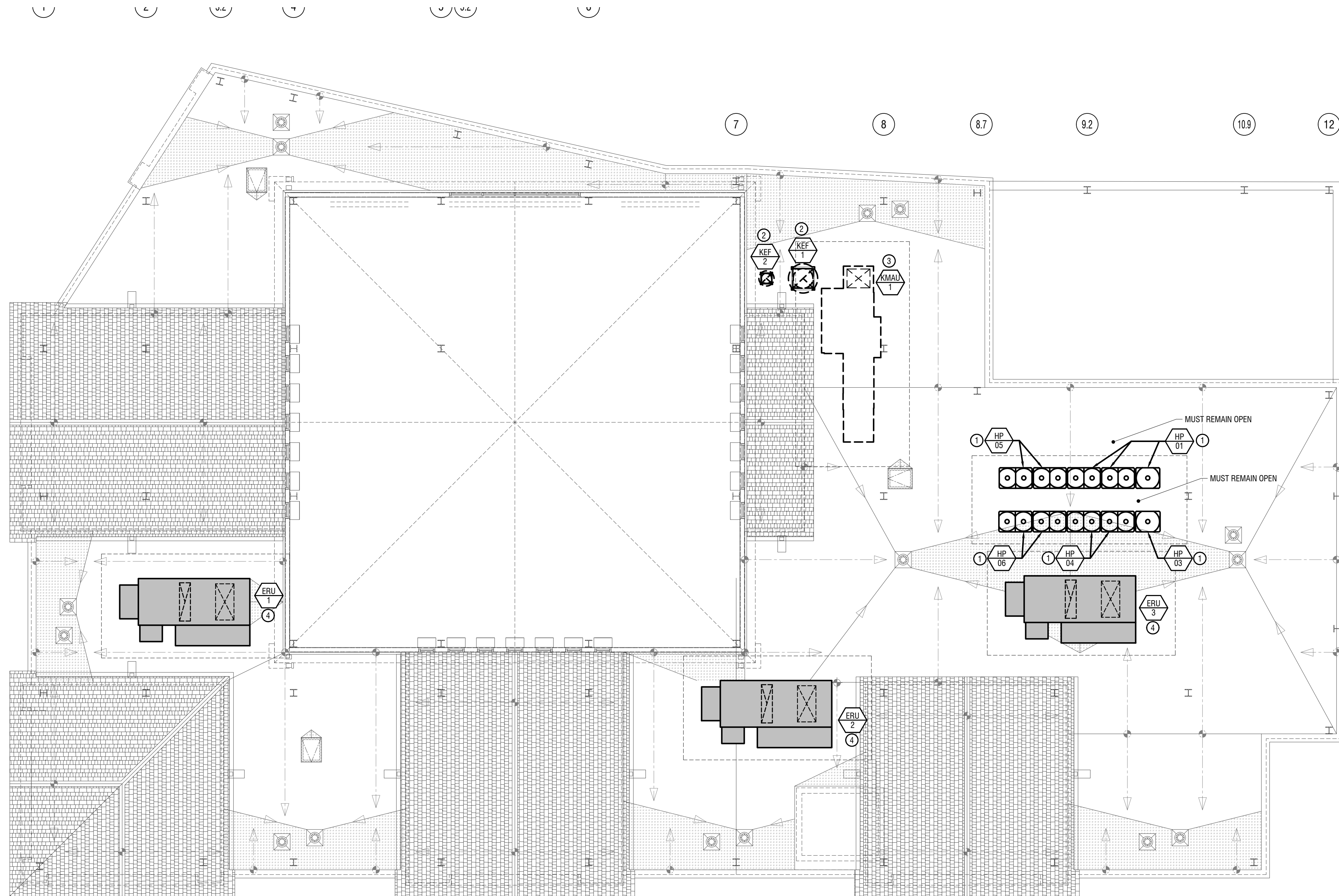
1 MECHANICAL PLAN - ROOF PLAN M2.4 SCALE: 1/8" = 1'-0"
