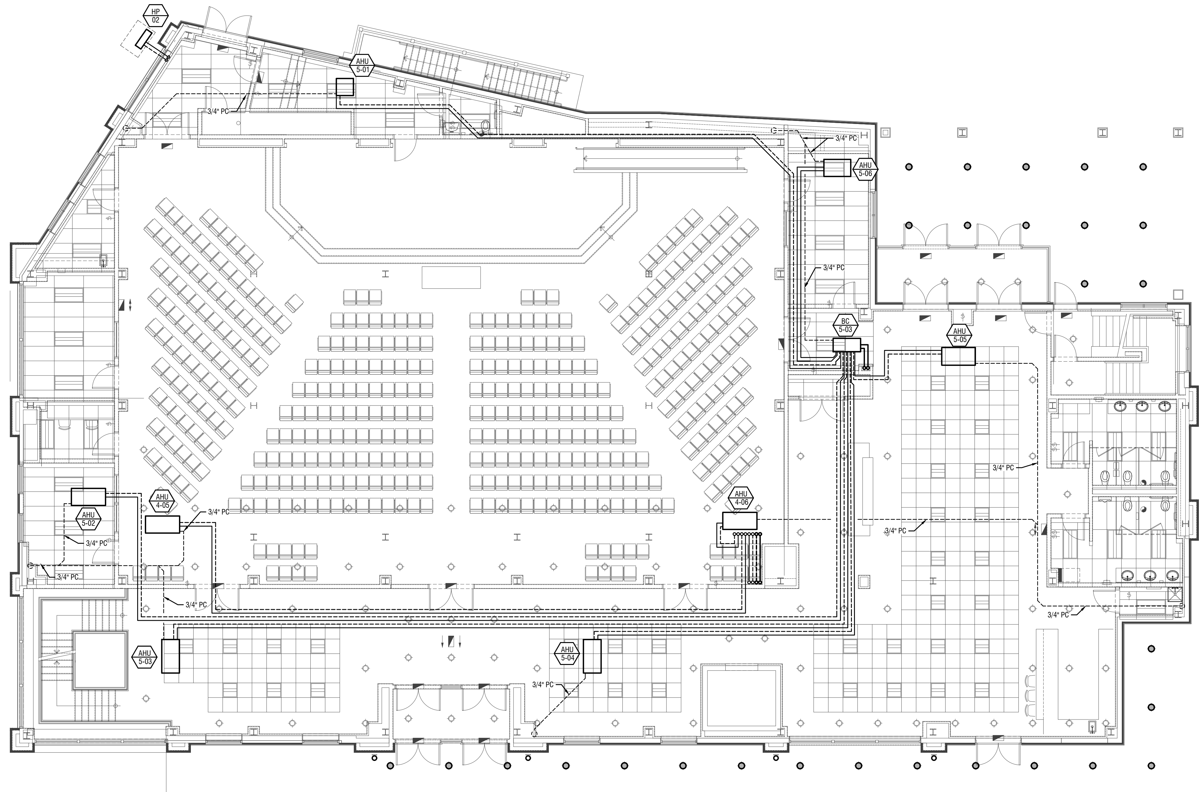
1 MECHANICAL PLAN - FIRST FLOOR M3.2 SCALE: 1/8" = 1'-0"
